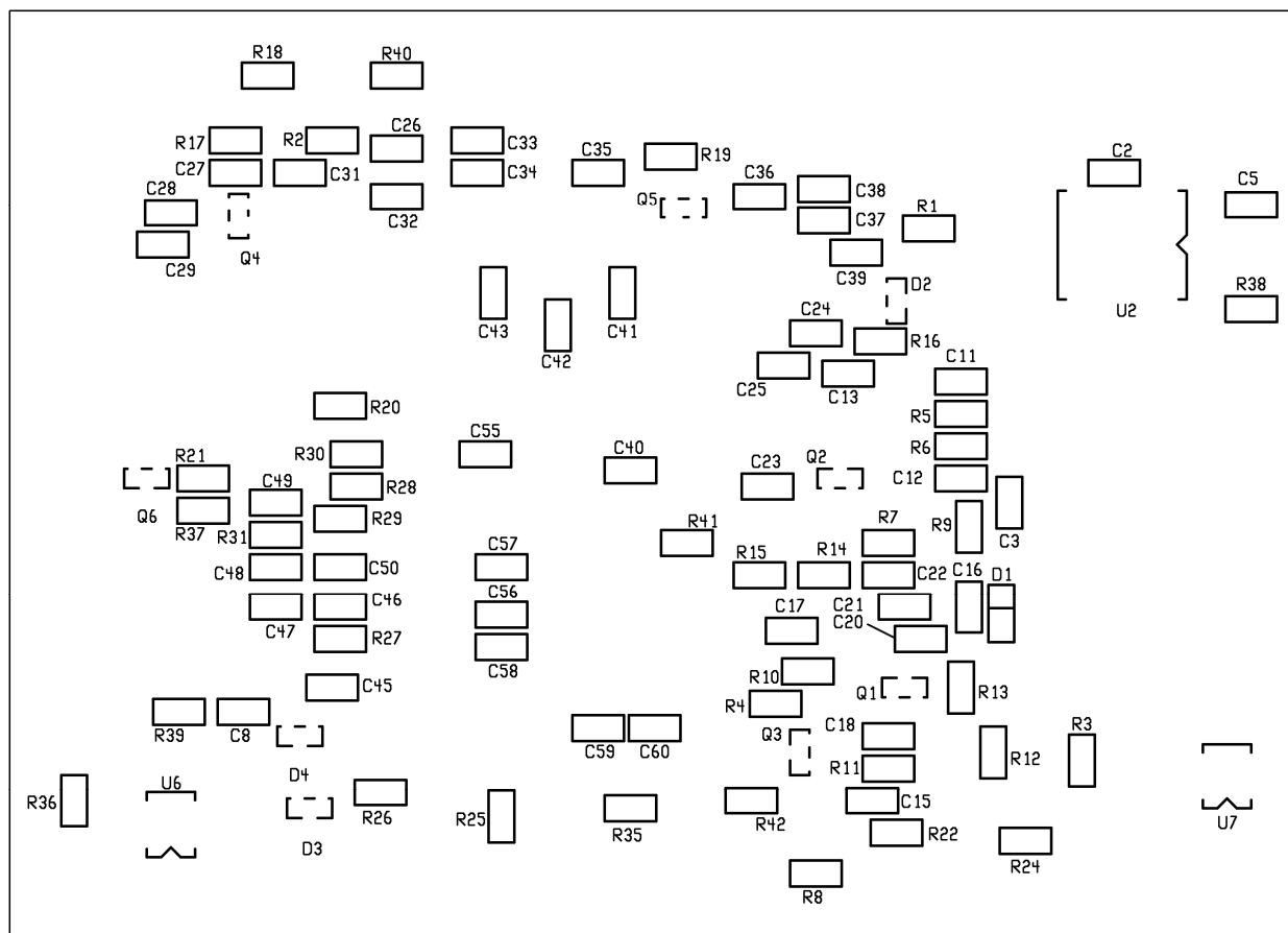
View of bottom of board.
